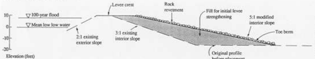
Constant-Slope Buttress
